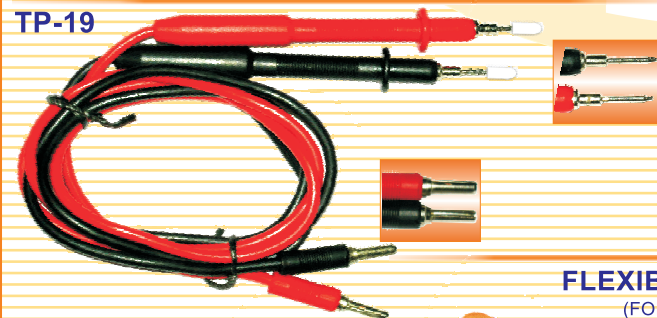
One end 2mm Soldered pin Other end 4mm spring action soldered pin
